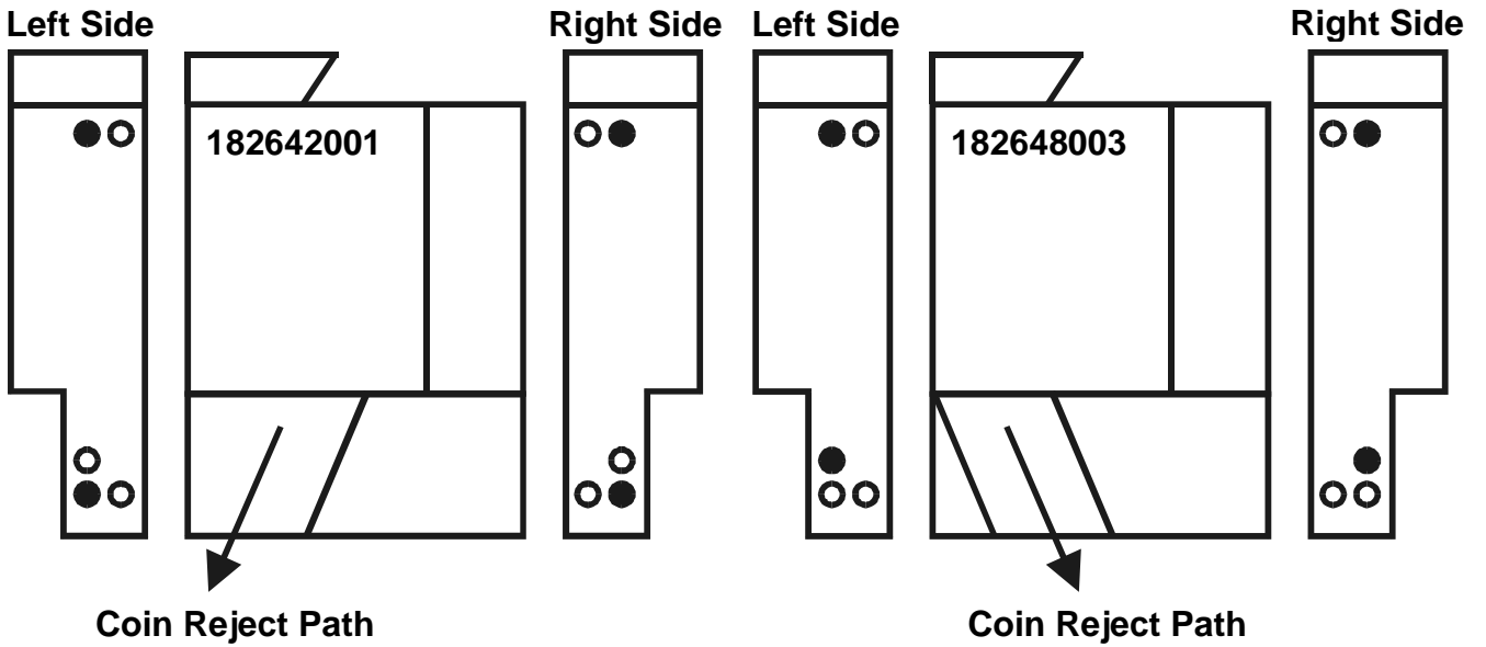
5" Adaptor (Type 1, Reject B)
